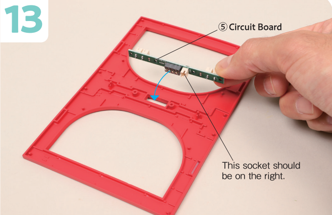
Assemble the ⑤ Circuit Board to the ① Ceiling Top Panel by fitting its terminal part into the opening in the Ceiling Top Panel.
