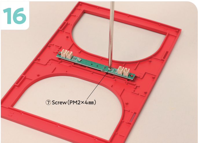
Tighten and secure another ⑦ Screw (PM2×4mm) into the remaining hole in the Circuit Board in the same manner.
