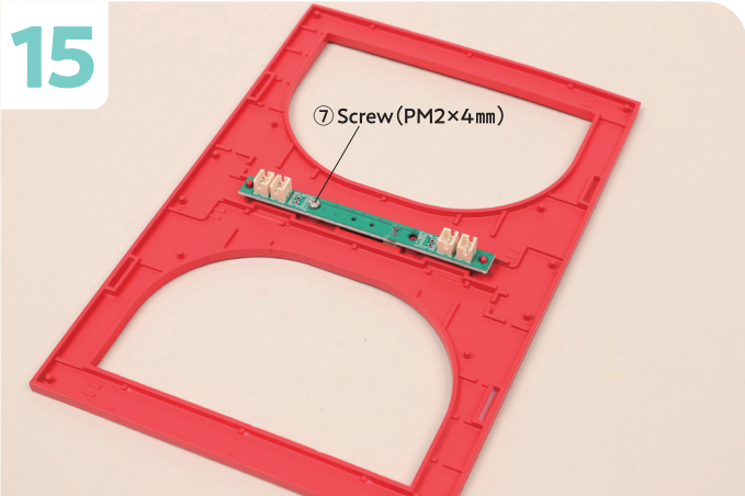
Tighten a ⑦ Screw (PM2×4mm) into the hole in the Circuit Board at the position indicated above.
