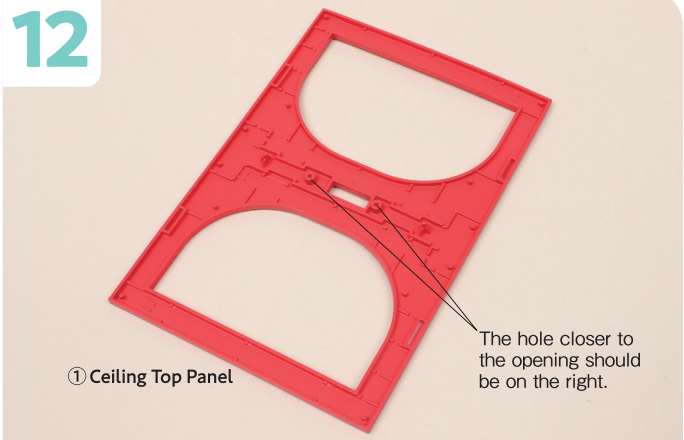
Check the orientation of the ① Ceiling Top Panel-the holes on either side of the rectangular opening in the middle are positioned differently. The hole closer to the opening should be on the right.
